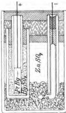
Abb. 69. Clark-Normalelement.
